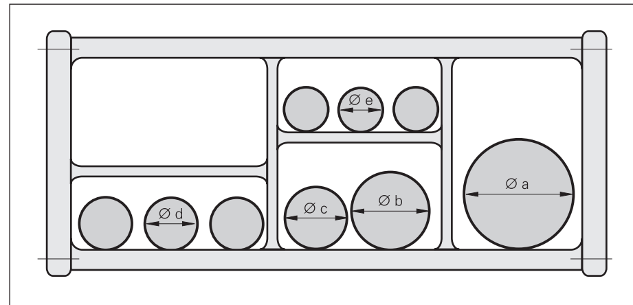
Configuration of a drag chain with cables of varying diameters (Ø x)
