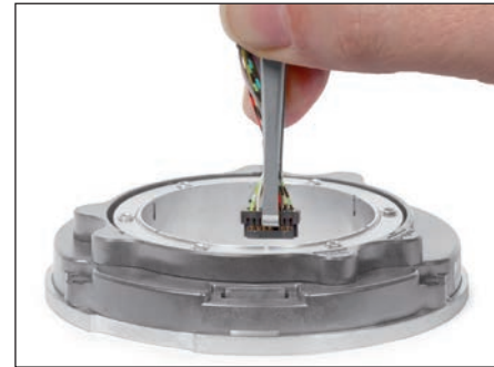
Mounting aid for output cable
