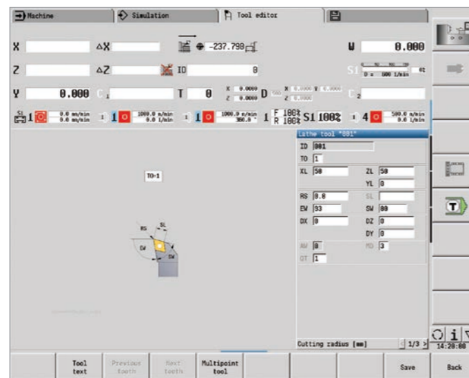
Tool editor
