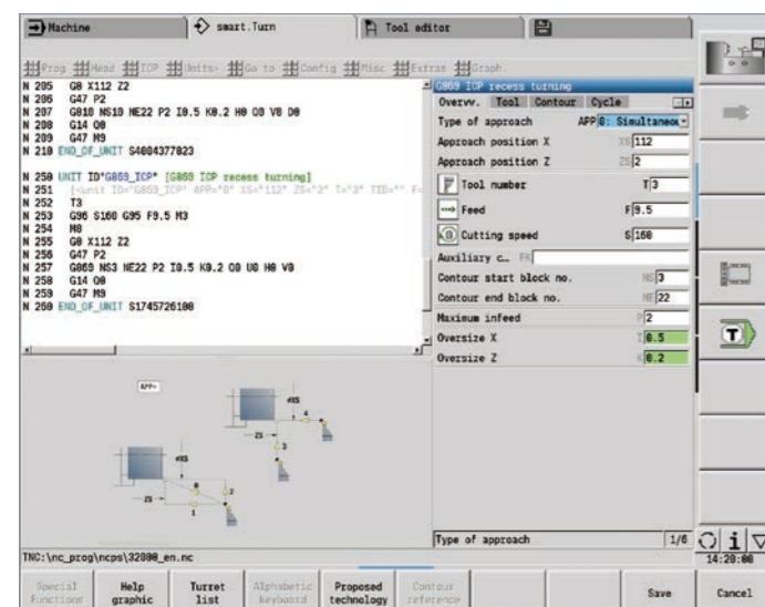
Input form in smart.Turn
