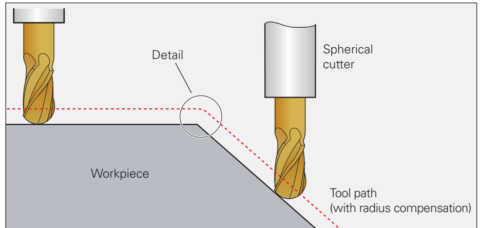
Figure 2: TCP tool path for a ball-nose cutter
